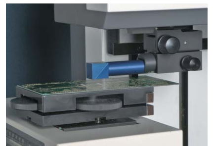
E-DT-SL-12B optical pickup
